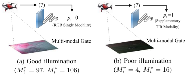
Fig. 3. Decision-making of multimodal gating.
