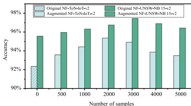
FIGURE 9 GraphACGAN's multi-classification accuracy on original and augmented datasets.
