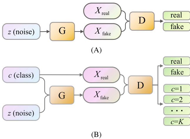
FIGURE 2 ACGAN versus GAN. (A) GAN framework and (B) ACGAN framework.
