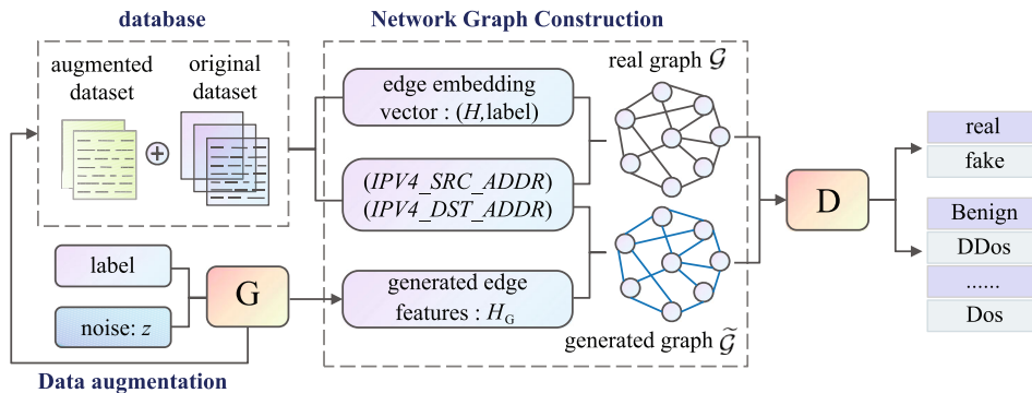
FIGURE 3 GraphACGAN intrusion detection framework.
