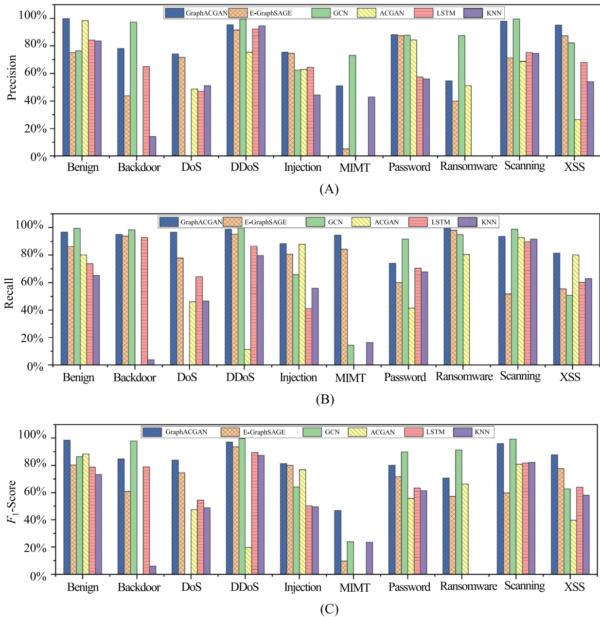
FIGURE 7 Multi-classification performance comparison on NF-ToN-IoT-v2. (A) Precision for each class, (B) recall for each class, and (C) F_1 -scores for each class.
