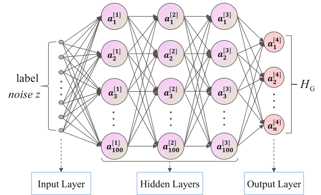
FIGURE 4 Generator network framework.
