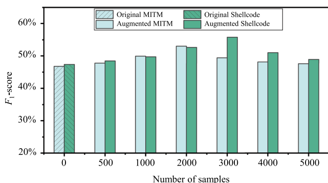
FIGURE 10 F_1 -scores for MIMT and Shellcode attacks on original and augmented datasets.
