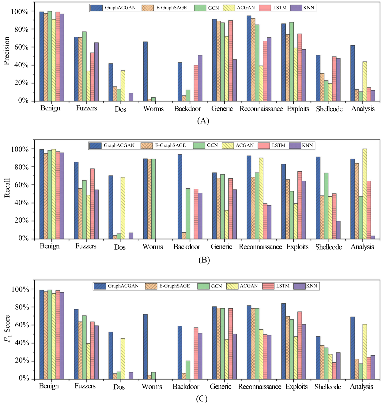
FIGURE 8 Multi-classification performance comparison on NF-UNSW-NB15-v2. (A) Precision for each class, (B) recall for each class, and (C) F_1 -scores for each class.
