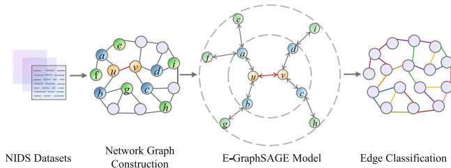
FIGURE 1 Edge classification based on E-GraphSAGE.
