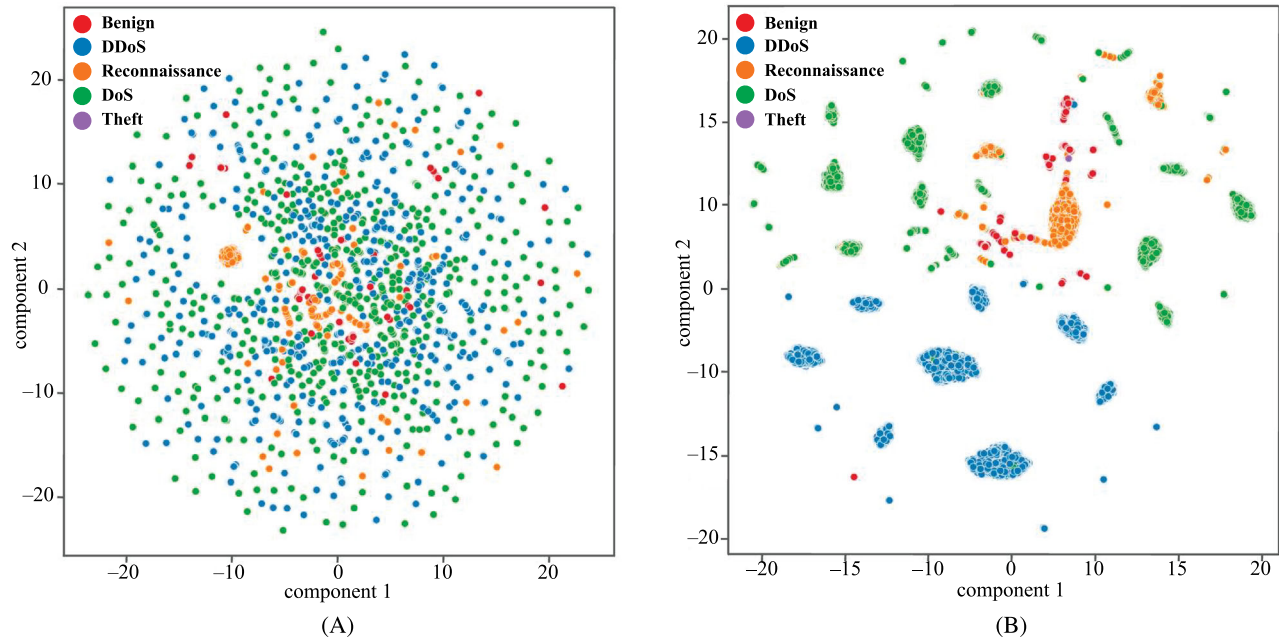
FIGURE 11 Visualization of attack traffic classification. (A) 10 000 random samples on NF-BoT-IoT-v2 and (B) separated high-dimensional edge features.
