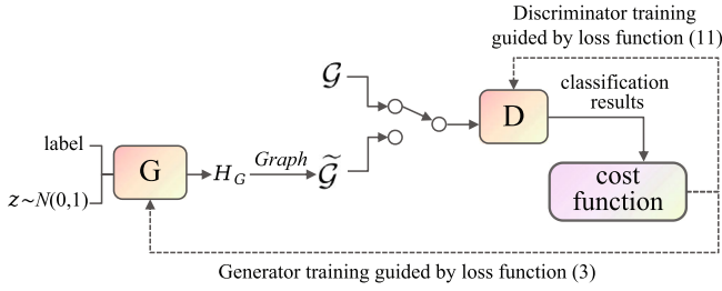
FIGURE 5 Algorithm workflow.
