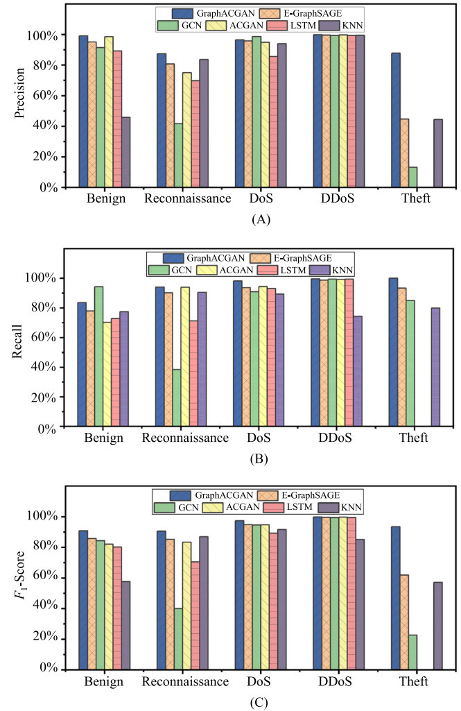
FIGURE 6 Multi-classification performance comparison on NF-BoT-IoT-v2. (A) Precision for each class, (B) recall for each class, and (C) F_1 -scores for each class.
